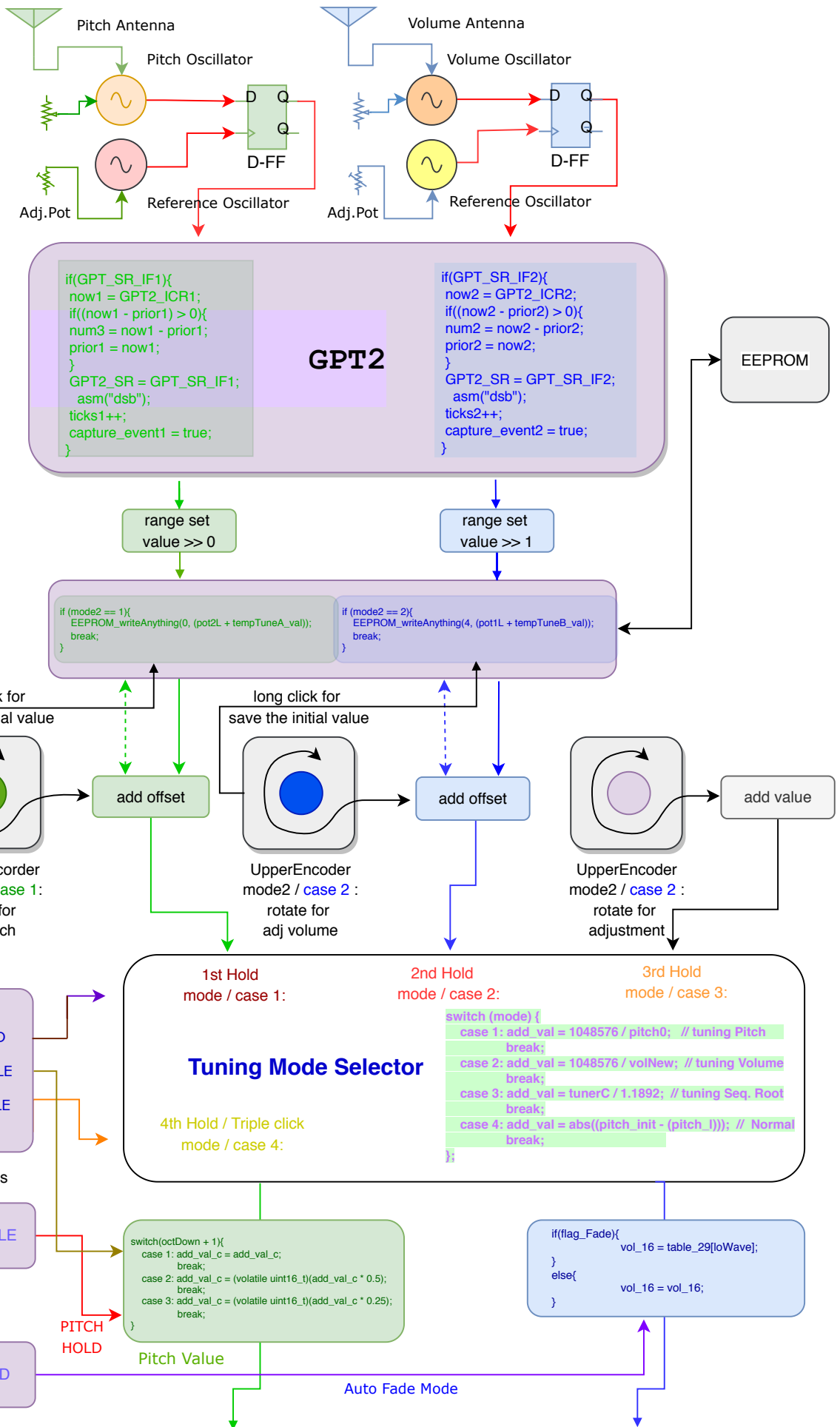
The signal flow around the Pitch/Volume Tuning System
